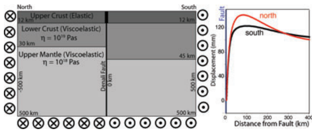
Figure 16. Finite-element model to investigate the asymmetry generated in the postsismic displacement field by differences in Moho depth. (a) Idealized rheological structure in cross-section normal to the fault. Displacements take place out of the plane of the cross-section. (b) Fault-parallel horizontal displacements predicted for the time period between 1.5 and 2.5 yr after the earthquake.
