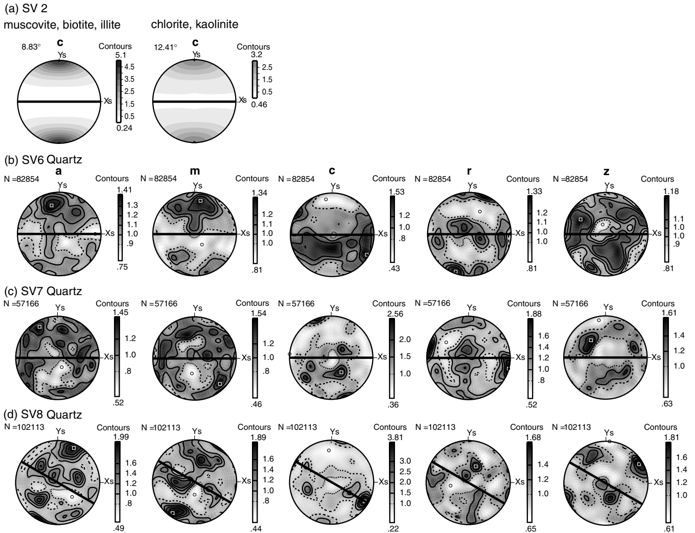
Figure 4. LPO for minerals in the shale (SV2) and sandstone (SV6, SV7, SV8) samples. The orientation of bedding is indicated by the thick black line. All contours are m.u.d.; maximum and minimum values are indicated by the solid black squares and open circles, respectively. (a) SV2: normalized transmission XTG-derived LPO for phyllosilicate and clay minerals: (left-hand panel) combined muscovite, biotite and illite; (right-hand panel) chlorite and kaolinite. (b) SV6: EBSD-derived LPO for quartz. (c) SV7: EBSD-derived LPO for quartz. (d) SV8: EBSD-derived LPO for quartz.
