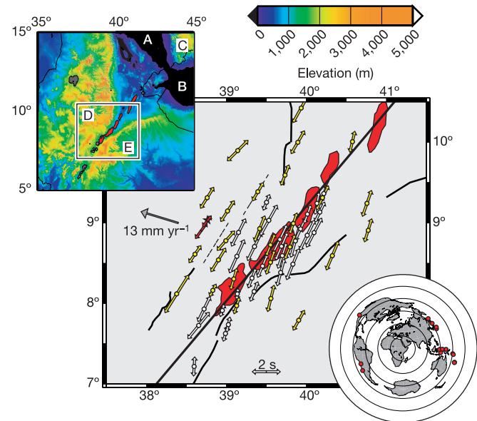
Figure 1 SKS splitting results in the region of the Northern Ethiopian Rift. The orientation of arrows shows the alignment of fast shear waves and the length of the arrow is proportional to the magnitude of the splitting. Yellow arrows mark results at seismic stations deployed for 16 months, white arrows are for stations deployed for three months, and red arrows are for the IRIS permanent stations FURI and AAE. In total, the results represent >350 splitting measurements. Heavy black lines show major border faults, dashed lines show monoclines and magmatic segments are marked in red. The solid black line bisecting the magmatic segments shows the approximate rift axis used to construct Fig. 2c and d. The top left inset shows the topography and magnetic segments in the region of interest (A, Red Sea; B, Gulf of Aden; C, Arabian plate; D, Nubian plate; E, Somalian plate). The lower right inset shows the locations of events used for shear-wave splitting analysis. Concentric circles mark 30^\circ increments in distance from the array.
