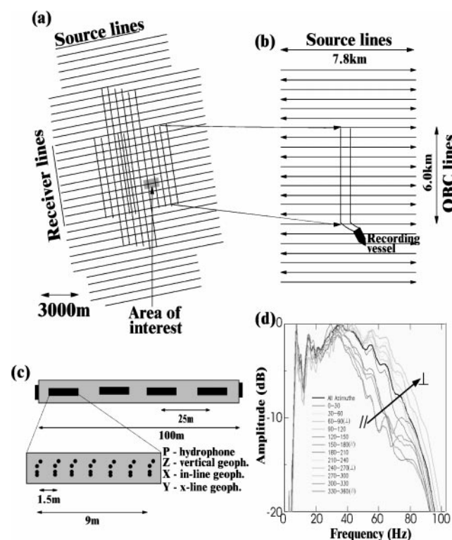
FIG. 3. Acquisition design for this OBC data example. (a) Orthogonal source- and receiver-line layout with 600-m spacing between each line. (b) Data acquired using patch shooting involving twenty-three, 7.8-km lines at 600 m spacing with shots every 25 m over pairs of receiver lines. (c) Receiver arrays positioned at 25 m along each 6-km receiver cable with seven, four-component sensors at 1.5 m spacing in each group. The area of interest for the anisotropy analysis is highlighted in (a). (d) Amplitude spectra for different azimuths bins (produced by Dave Wilson, BP, 1999); the receiver line parallel (//) direction is approximately 350^\circ/170^\circ . Above about 35 Hz, there is significant variation in the frequency content along the different azimuths. This is from a previously applied summation of the seven receivers in each array providing an azimuth-dependent array filter that cuts out more of the higher frequencies in the direction parallel to the array than perpendicular to it.
