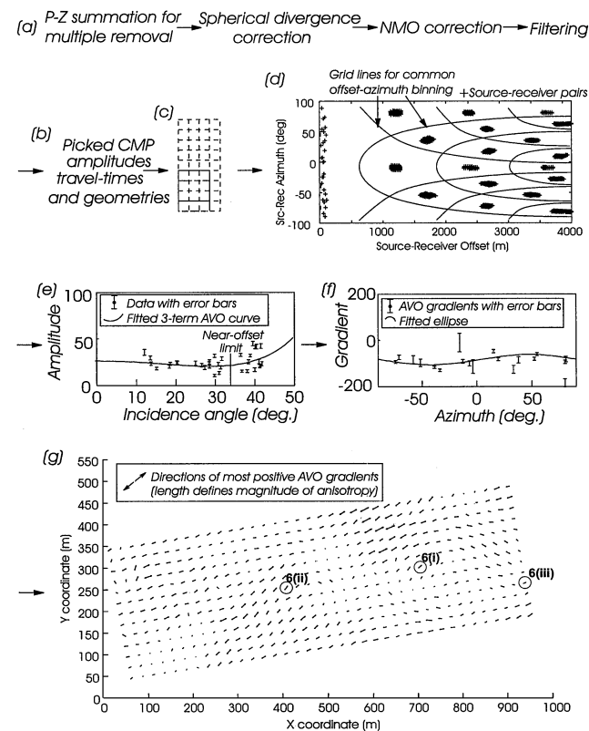
FIG. 4. Schematic representation of the processing flow for AVOA analysis of 3D OBS data. (a) Standard preprocessing to improve the primary reflections. (b) Amplitudes and traveltimes are picked in the CMP gathers and labelled with the CMP geometry data. (c) These amplitude and time data are regrouped into overlapping 75 \times 75 -m CMP gathers and binned to common offset-azimuth groups with offset and azimuth positions also averaged. (d) A 2D, Shuey-type AVO curve is fitted to the amplitude data to define the normal incidence amplitude and near-offset range. (e) These values are used to define the azimuthal variation in the near-offset AVO gradients for each of the 75 \times 75 -m data gathers. The gradients will have an elliptical variation with azimuth so an anisotropy ellipse can be determined. (g) The major axes of the near-offset AVO gradient ellipse for each CMP are plotted in map form to provide insight into fracture orientations and their spatial variability. The CMP locations of the AVOA data examples of Figure 6(i)–(iii) are also indicated. Note that a similar approach is applied for traveltimes but using NMO velocity rather than AVO gradient.
