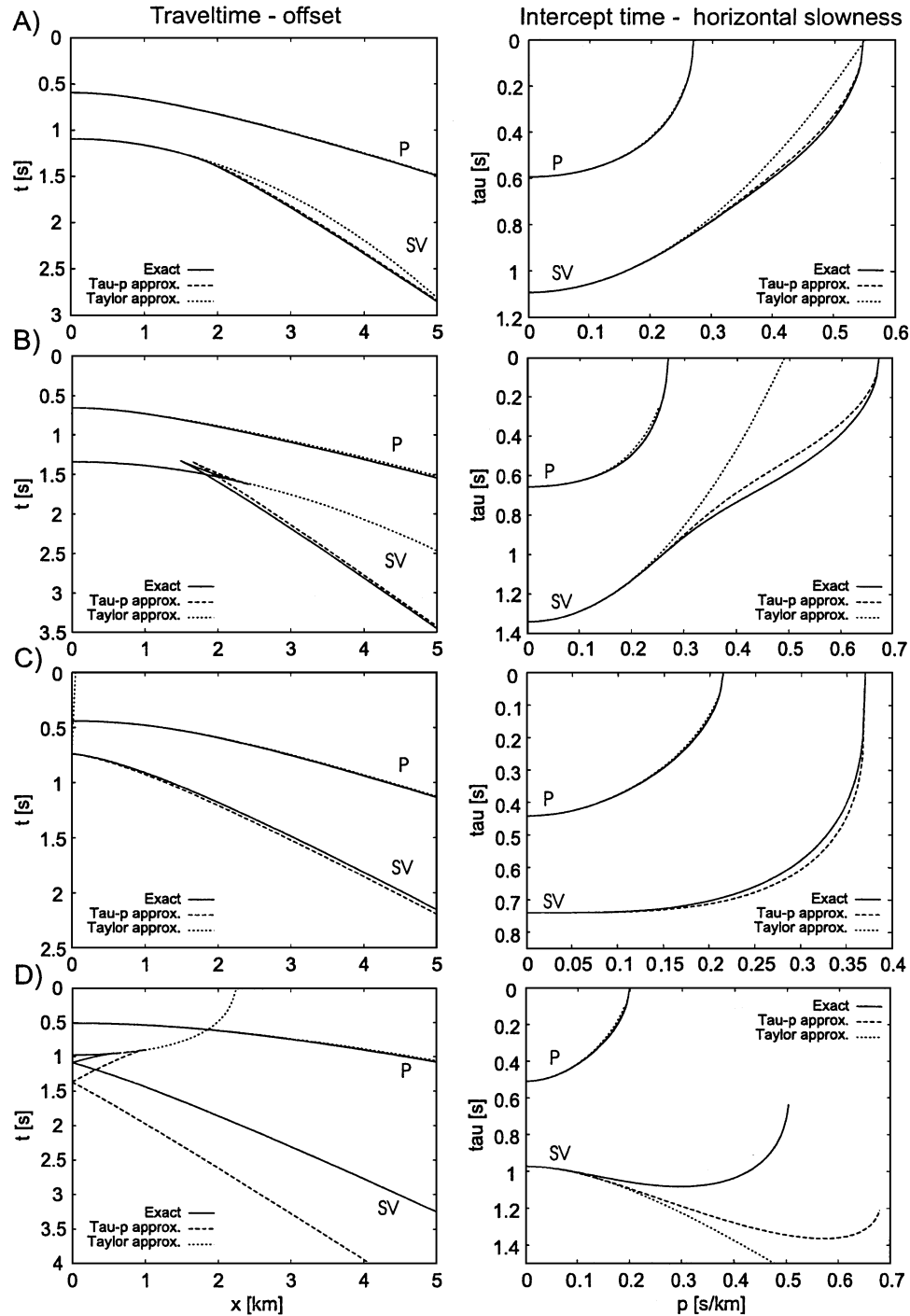
FIG. 2. Moveout (left) and \tau(p_x) curves (right) associated with 1-km-thick packages of shales A, B, C, and D. Solid line: exact curves; long dashes: \tau - p method using reduced-parameter expressions; short dashes: Taylor series approximation.
