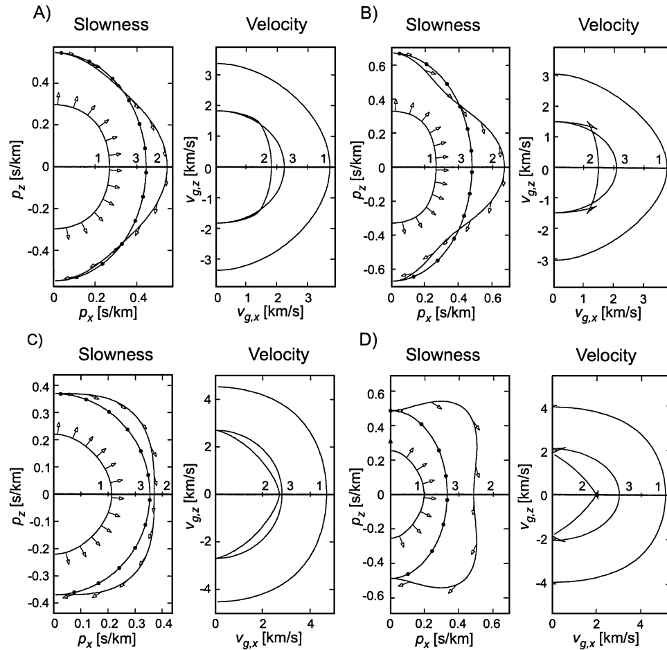
FIG. 1. Phase-slowness (left) and group-velocity (right) surfaces of the four shales A, B, C, and D considered in the numerical examples. Arrows indicate polarisations. Numbers 1 = P , 2 = SV , 3 = SH . See Table 1 for the elastic coefficients.
