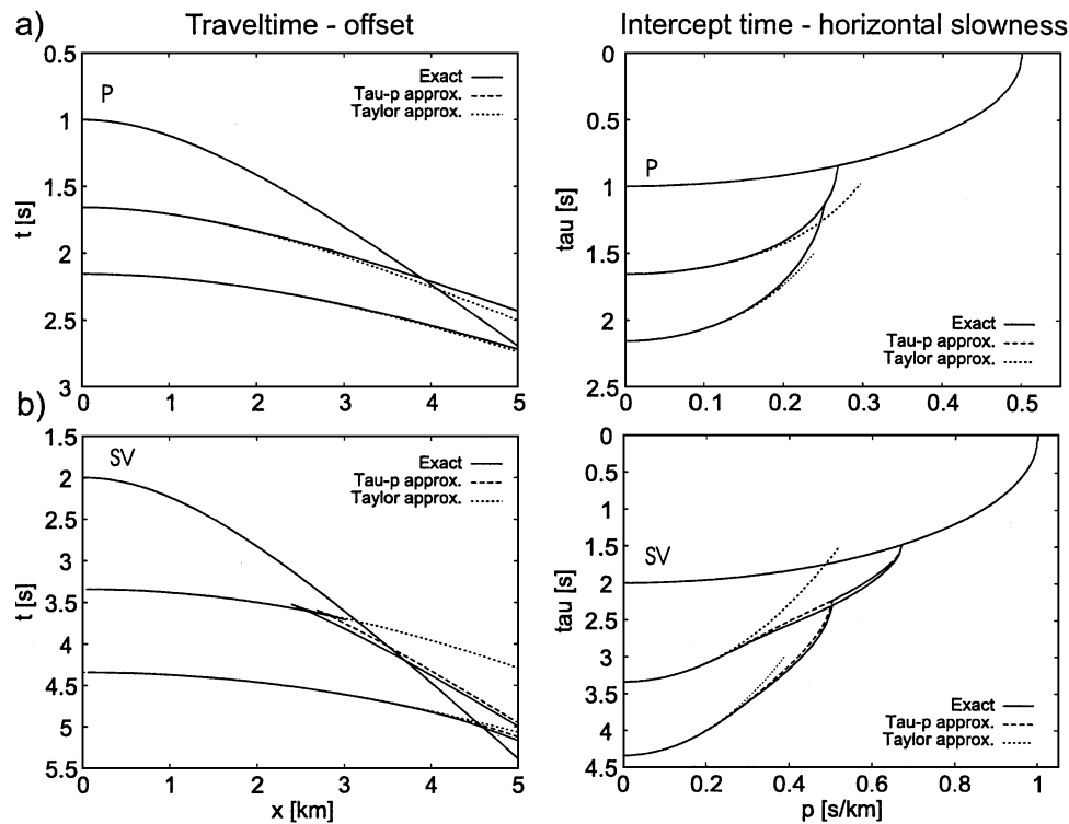
FIG. 3. Moveout and \tau(p_x) curves of the three-layer model for (a) P -waves and (b) SV -waves. Only the second layer is anisotropic (shale B). Solid line: exact curves; long dashes: \tau - p method using reduced-parameter expressions; short dashes: Taylor series approximation.
