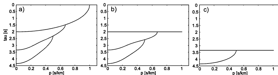
FIG. 4. Layer stripping in the \tau - p domain: (a) \tau(p_x) curves of all three SV -waves [identical to the exact curves in Figure 3b (right column)], (b) first layer removed, and (c) top two layers removed.
