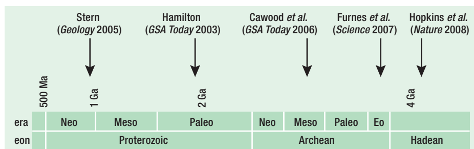
2: Estimates of when plate tectonics began on Earth. (Based on the studies of Stern 2005, Hamilton 2003, Cawood et al. 2006, Furnes et al. 2007 and Hopkins et al. 2008)
