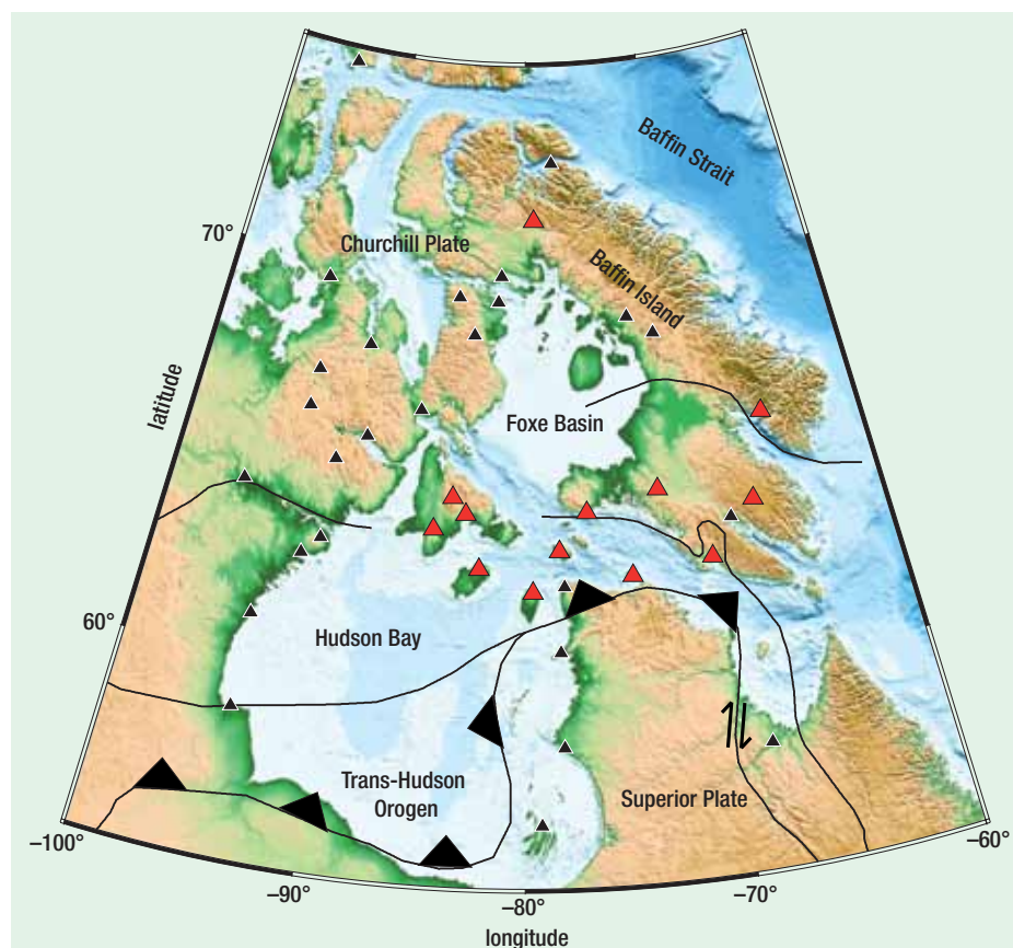
3: Seismograph stations in the Canadian north. The HuBLE-UK NERC stations (red triangles) lie within the footprint of the broader POLARIS (Eaton et al. 2005) and earlier seismograph networks (small black triangles). Dark lines show ancient plate boundaries.
